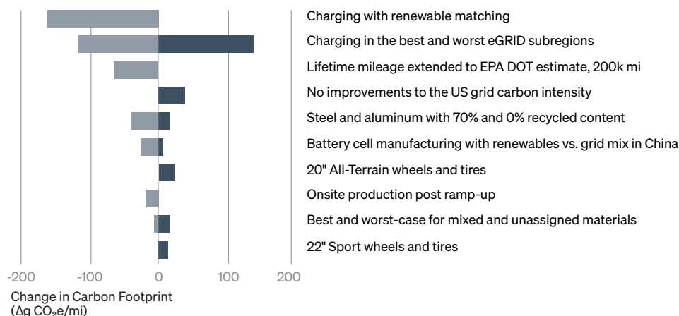
Figure 4 R1S Launch Edition carbon footprint scenario analyses
